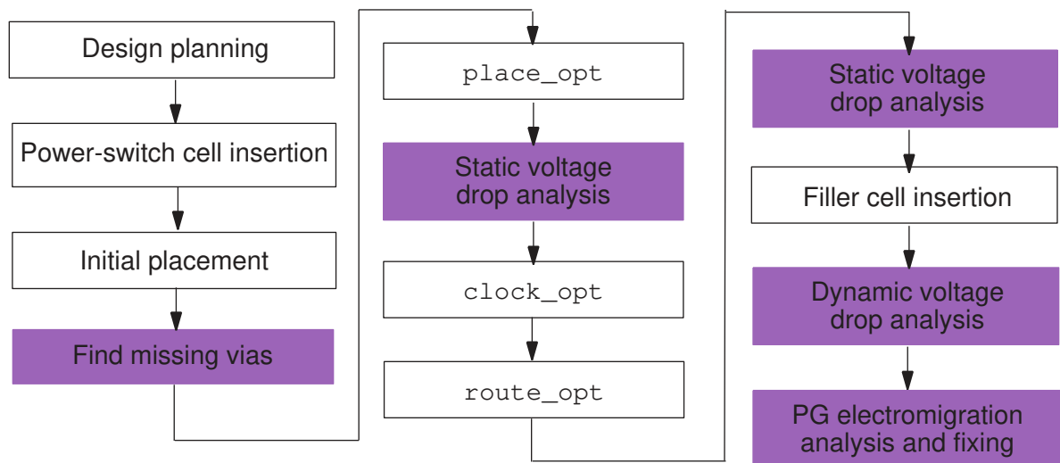
Figure 198 Using RedHawk Fusion in the Fusion Compiler Design Flow
