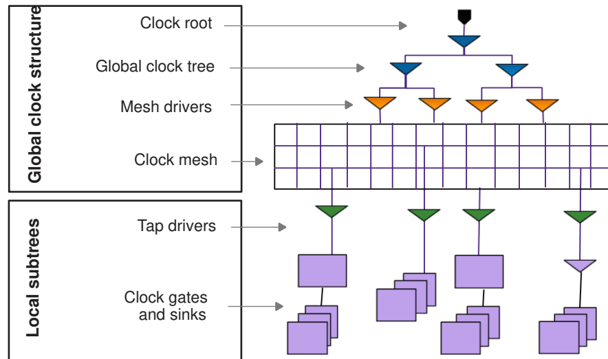
Figure 83 Regular Multisource Clock Tree
