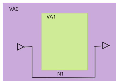
Figure 19 Physical-Feedthrough Nets Disabled for a Voltage Area
