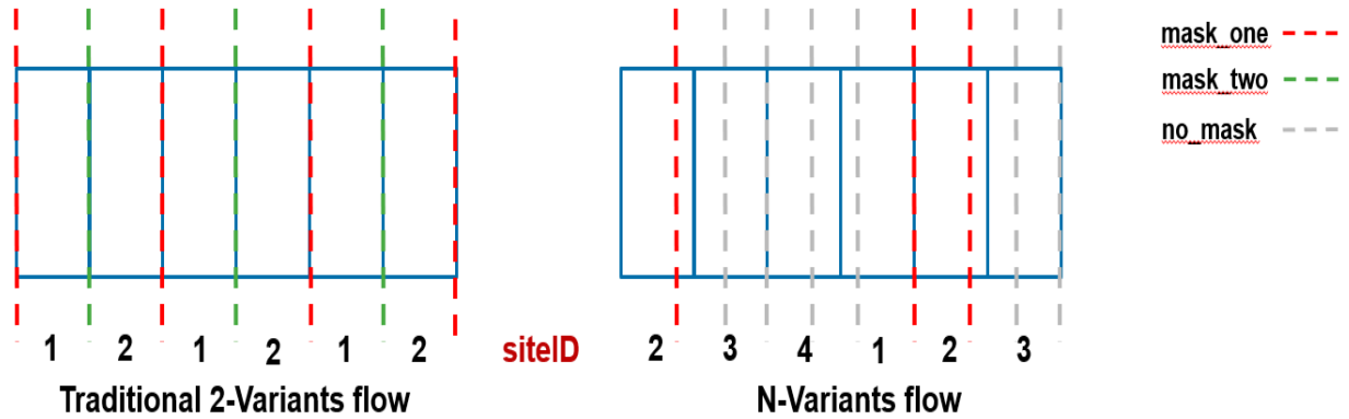
Figure 225 2-Variants and N-Variants Sub Flows in siteld_based Mode design with various tracks and pitches
