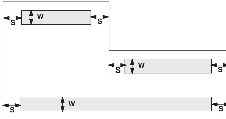
Figure 101 Continuous Metal Shape Perimeter Constraint Objects
