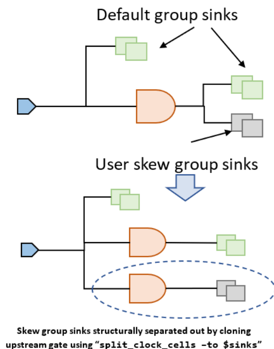
Figure 79 Faster Clock Tree to Specific Endpoints
