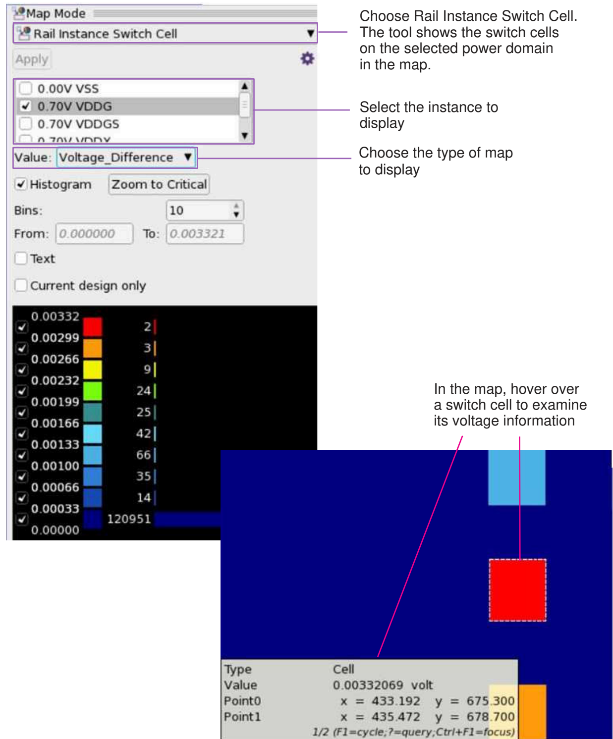
Figure 213 Displaying Maps for Switch Cells
