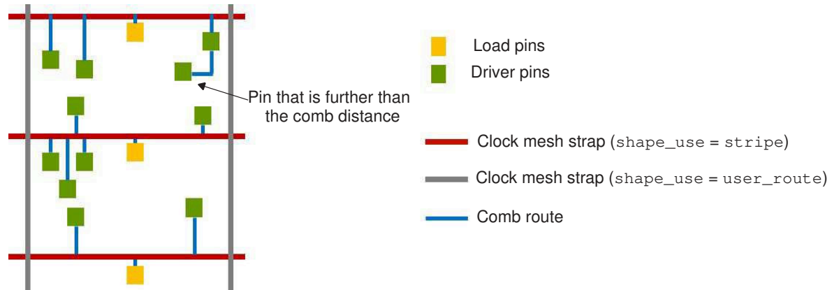
Figure 94 Comb Topology
