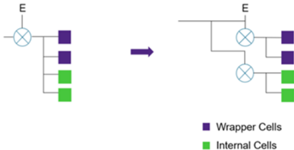
Figure 69 Splitting a Clock Gate to Internal Cells and Wrapper Cells
