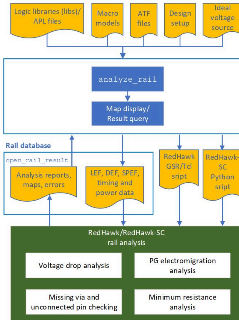
Figure 199 RedHawk Fusion and RedHawk-SC Fusion Data Flow
