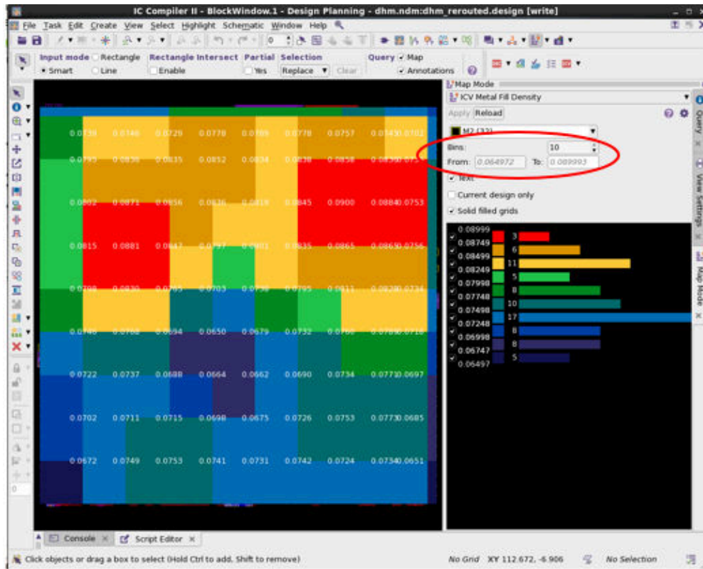
Figure 151 Minimum Density Heat Map
