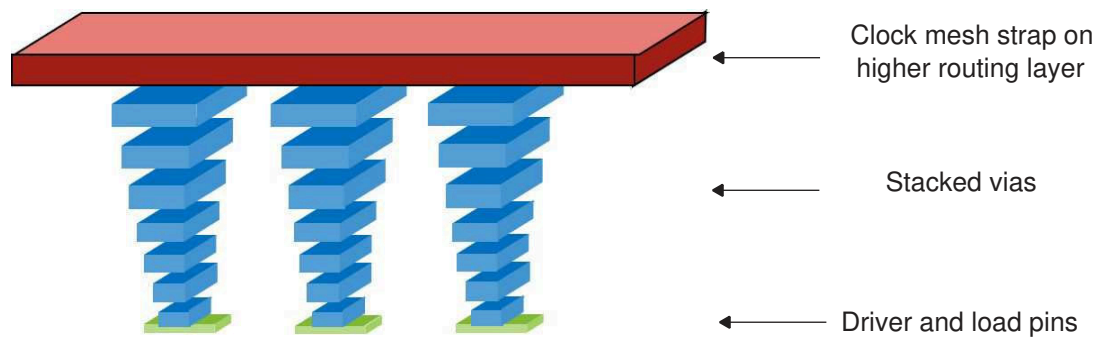
Figure 95 Vias in the Comb Topology
