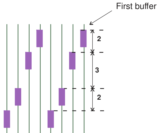
Figure 220 Buffer Patterns for a Vertical Bus
