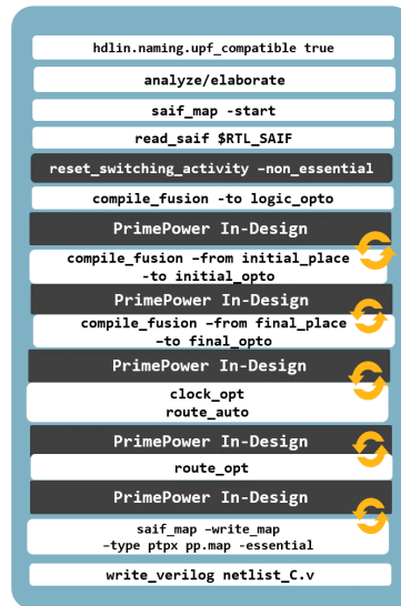
Figure 26 The PrimePower In-Design Flow
