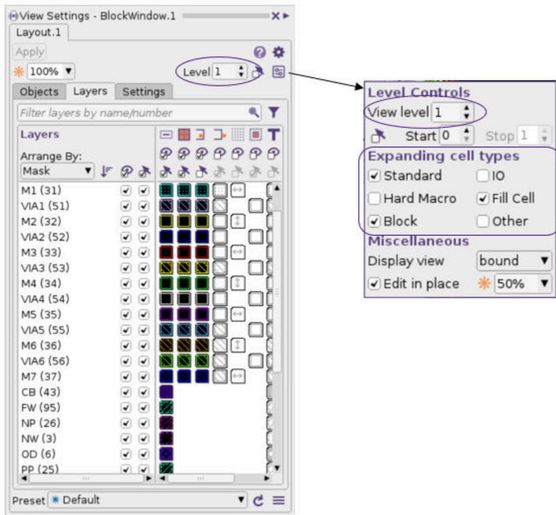
Figure 146 Settings Used to Display Objects for Design Rule Checking
