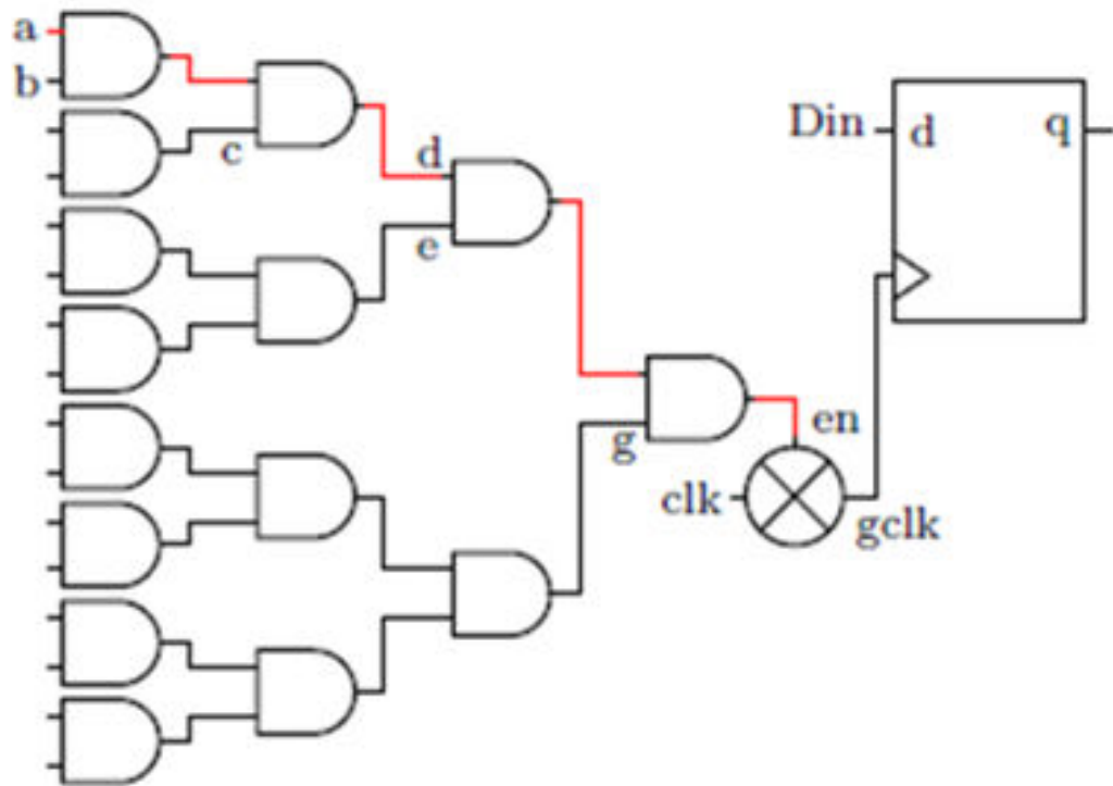
(a) Before enable exclusion. Signal a is to be excluded
