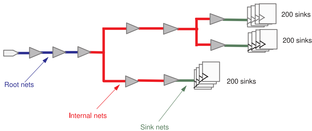
Figure 27 Root, Internal, and Sink Clock Net Types
