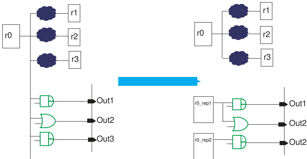
Figure 34 Using the -driven_by_original_register Option
