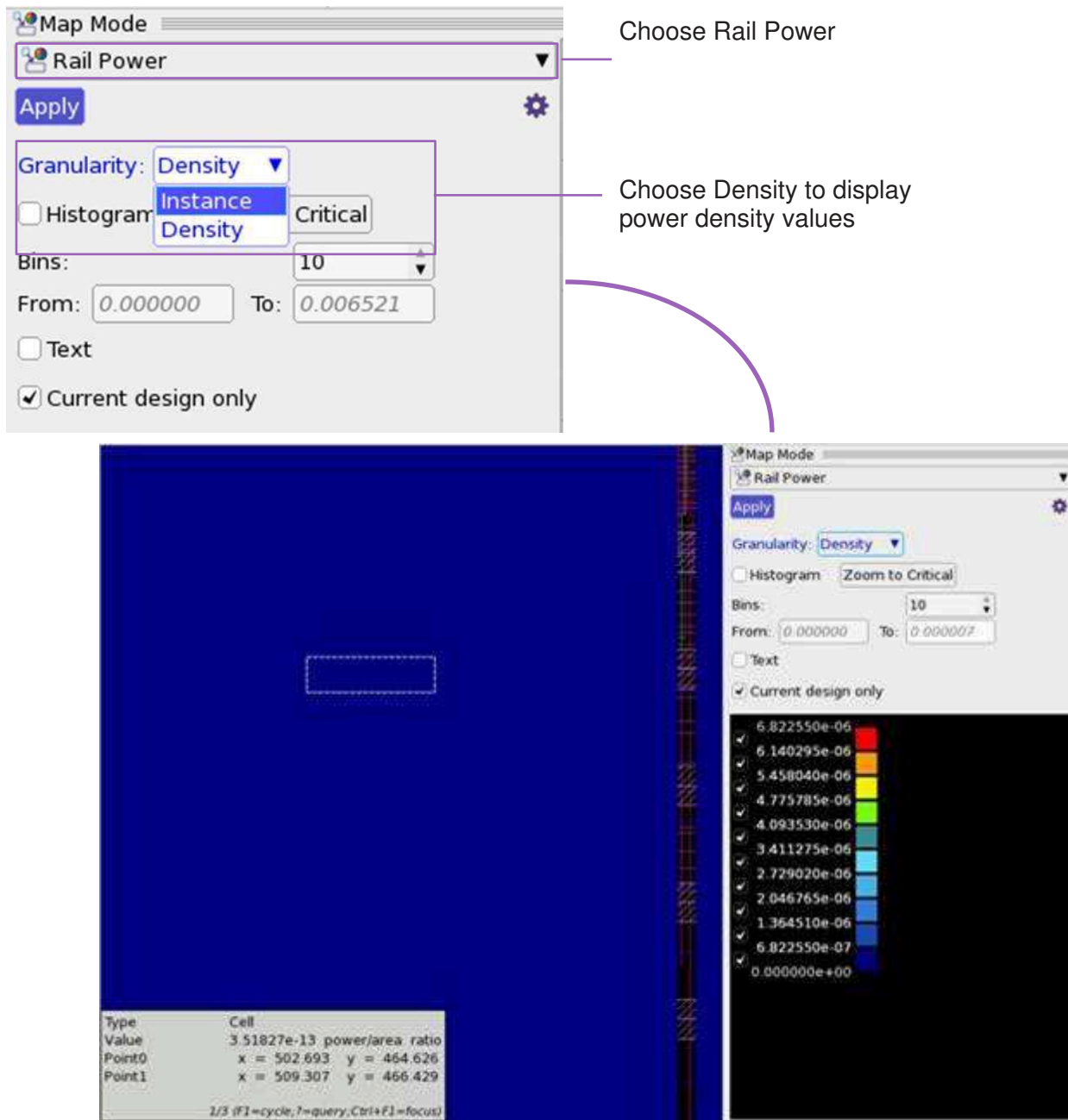
Figure 214 Displaying a Power Density Map
