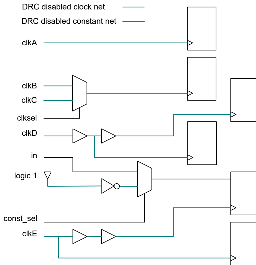
Figure 25 DRC Disabled Clock and Constant Nets Highlighted
