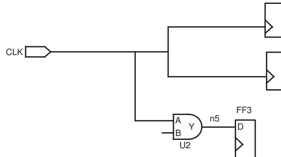
Figure 75 Specifying Exceptions on Pins Beyond the Clock Network
