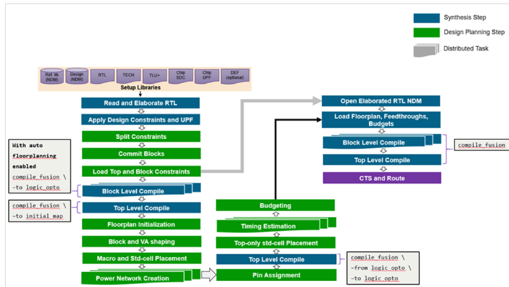
Figure 187 Hierarchical Synthesis Flow When Floorplans are not Available
