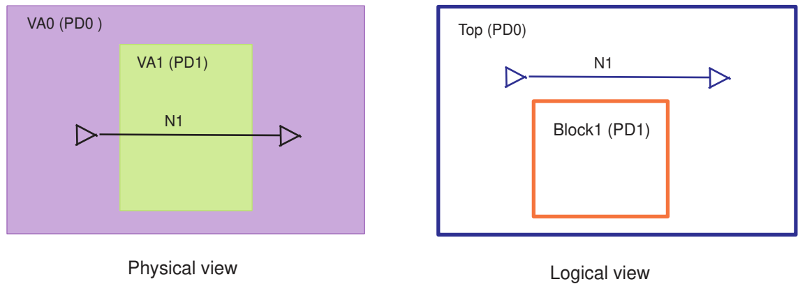
Figure 18 Physical-Feedthrough Nets of Voltage Areas
