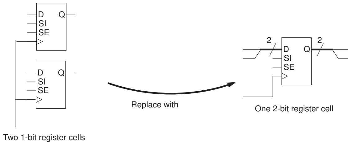
Figure 35 Replacing Multiple Single-Bit Register Cells With a Multibit Register Cell
