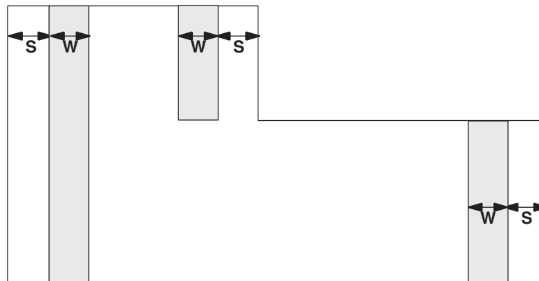
Figure 104 Routing Guide Perimeter Constraint Objects
