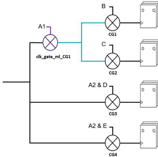
Figure 59 After Clock-Gate Level Expansion
