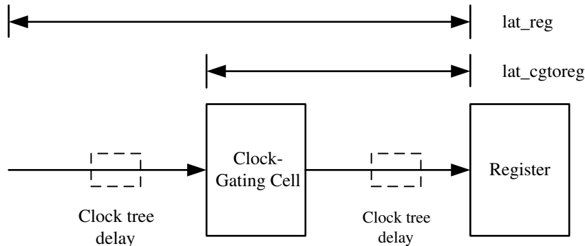
Figure 55 Clock Latency With Clock-Gating Design
