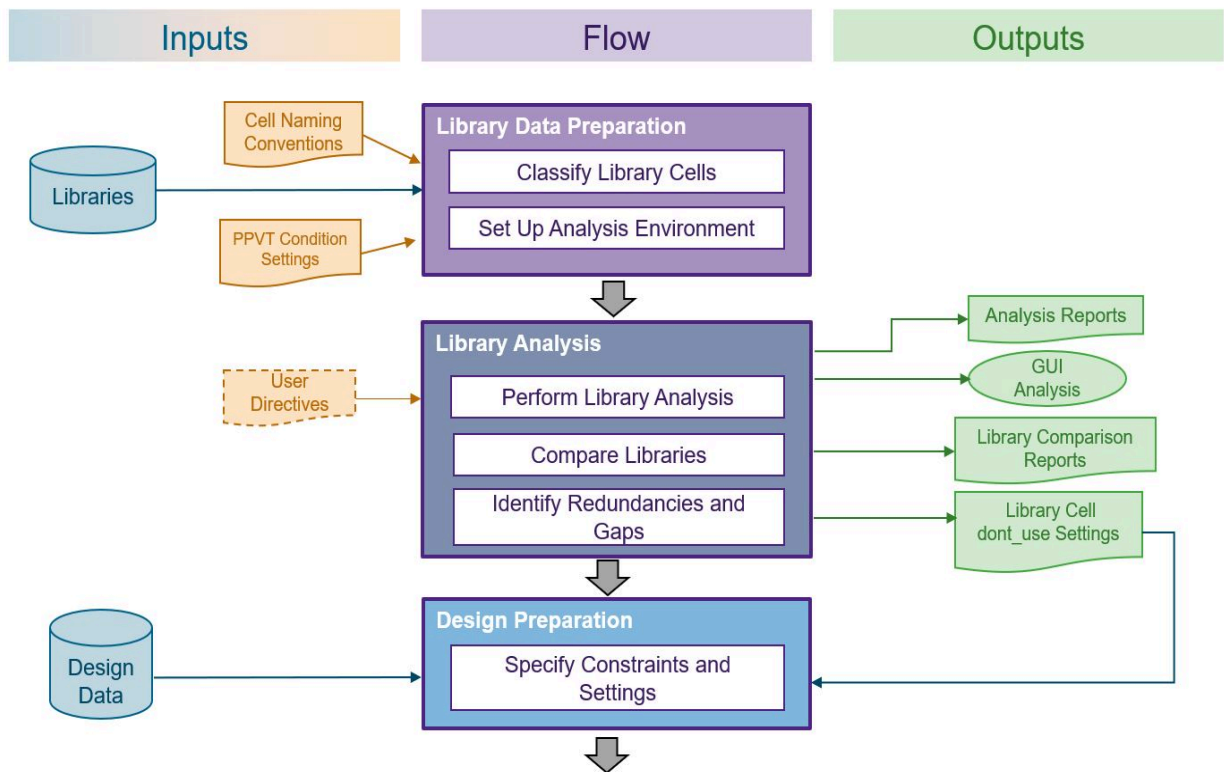
Figure 8 Library Analysis Flow
