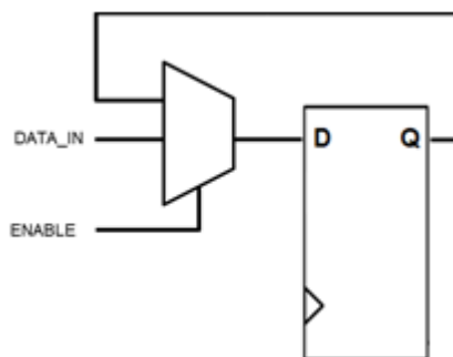
Figure 49 Enable Signal in a Feedback Loop
