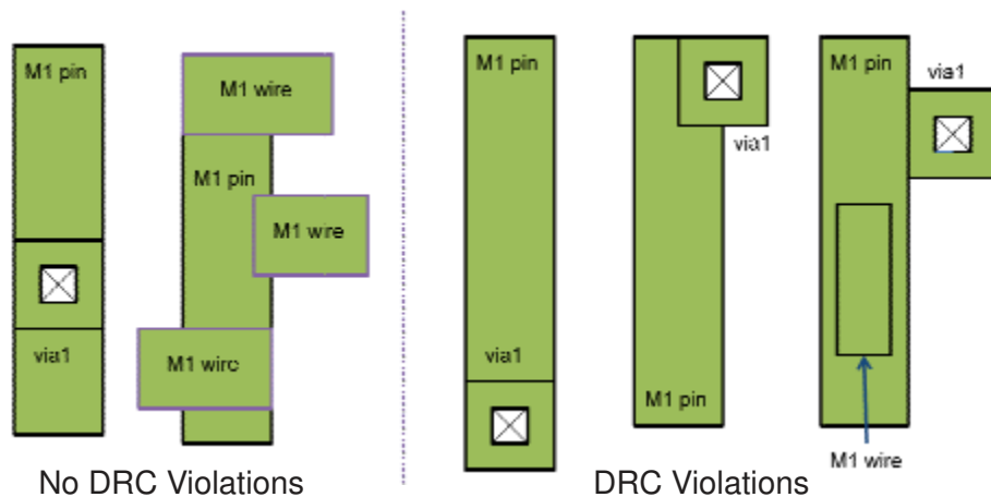
Figure 114 Restricted Via-to-Pin Connections
