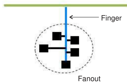
Figure 92 Fanout of a Finger of the Fishbone Topology
