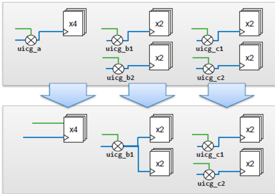
Figure 60 Example of Clock Gating Restrictions
