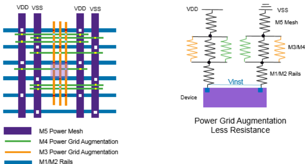
Figure 148 Power Grid Augmentation
