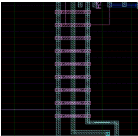
Figure 116 Coaxial Shielding
