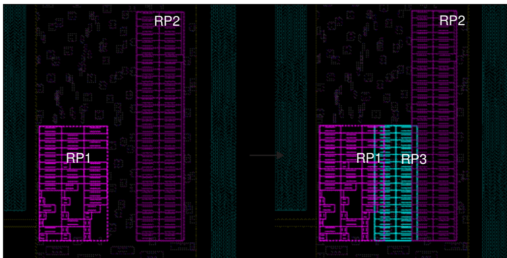
Figure 186 Legalizing the RP3 Relative Placement Group Over Other Groups
