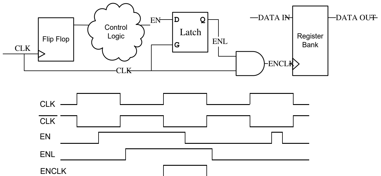
Figure 46 Latch-Based Clock Gating
