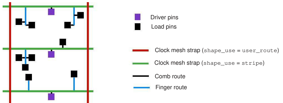
Figure 91 Fishbone Topology
