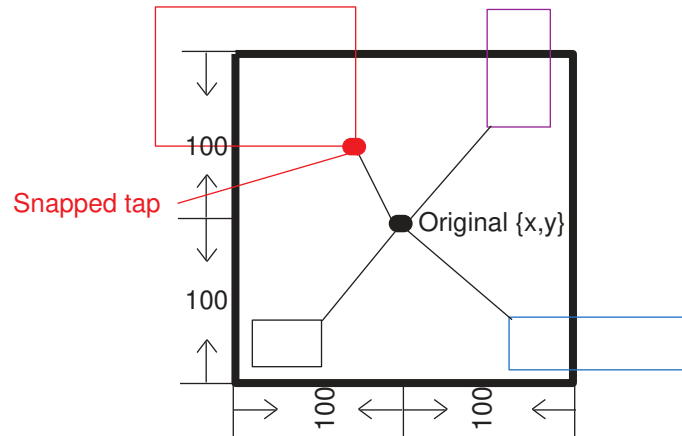
Figure 201 Finding a Substitute Location for an Invalid Tap
