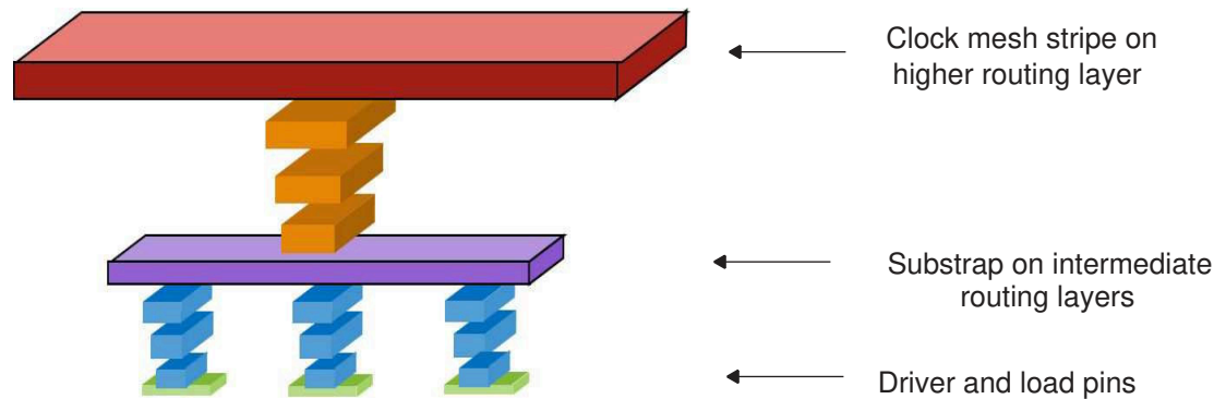
Figure 96 Vias in the Substrap Topology
