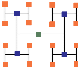
Figure 88 Clock Drivers Placed in an H-Tree Structure
