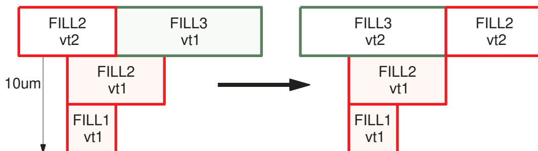
Figure 132 Fixing Maximum Stacking Violation by Reordering
