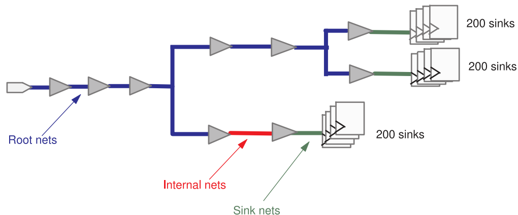
Figure 28 Using a Fanout Limit for Selecting Root Nets
