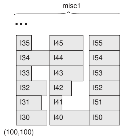
Figure 173 Anchored Relative Placement Group
