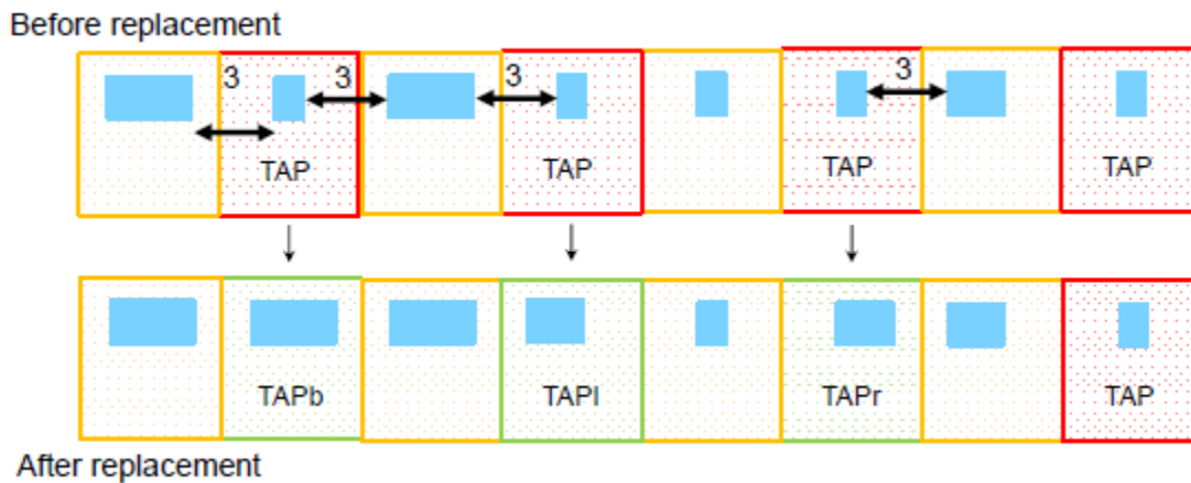
Figure 134 Fixing a Tap Cell Spacing Violation
