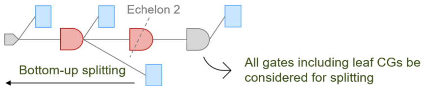
Figure 80 Latency Driven Clock-Gate Splitting
