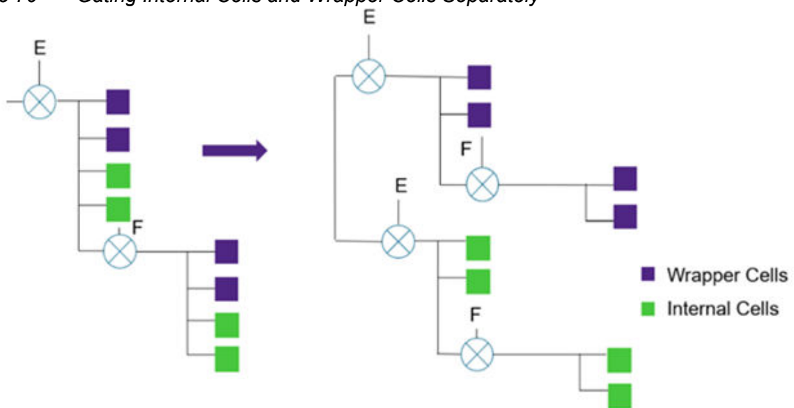
Figure 70 Gating Internal Cells and Wrapper Cells Separately
