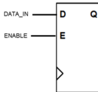
Figure 48 Directly Connected Enable Signal
