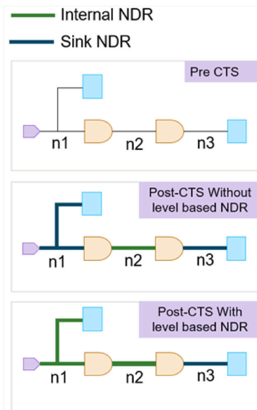
Figure 29 Level-Based Clock Nondefault Routing Rule
