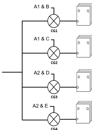
Figure 58 Before Clock-Gate Level Expansion
