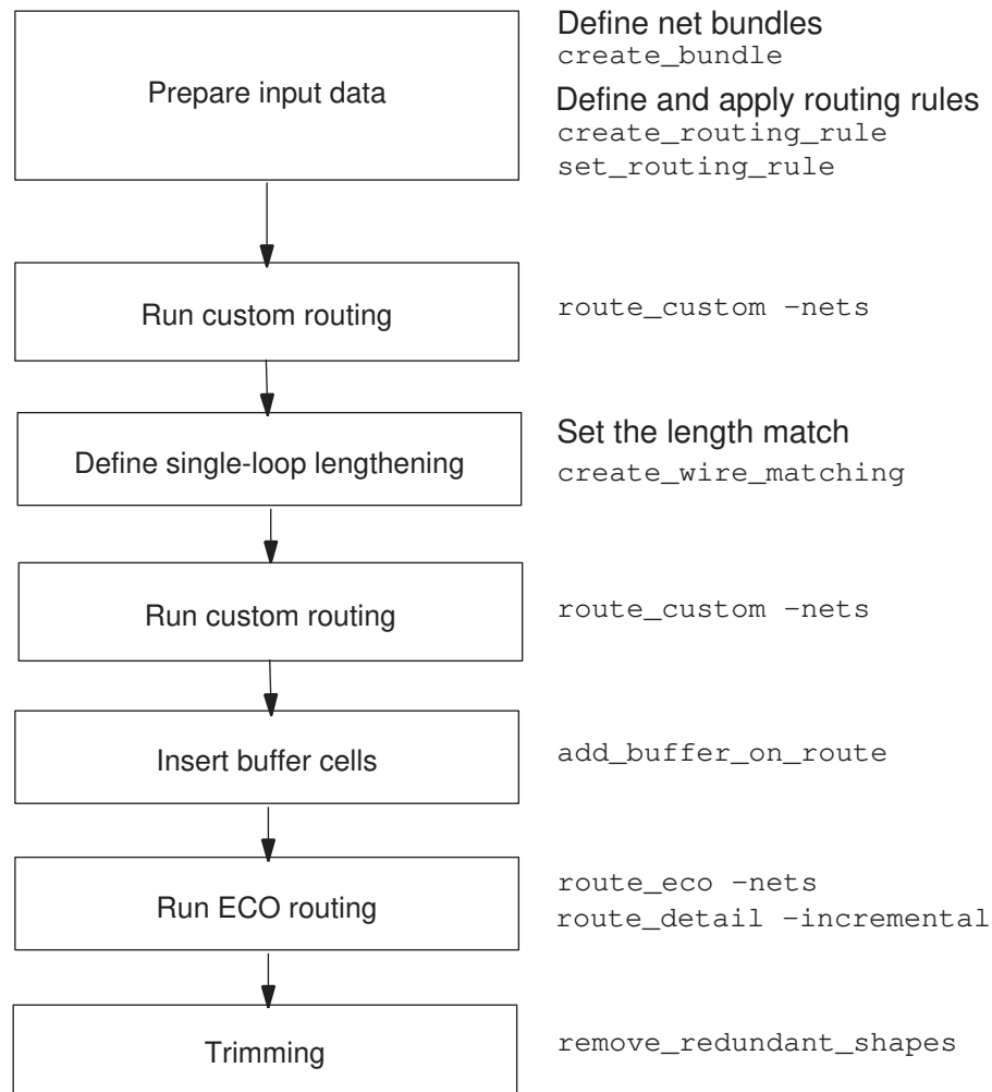
Figure 165 A Basic DDR Flow
