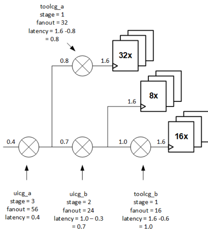
Figure 57 Latency Calculations With Varying Fanout
