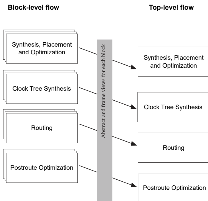
Figure 196 Top and Block Levels Implemented in Parallel
