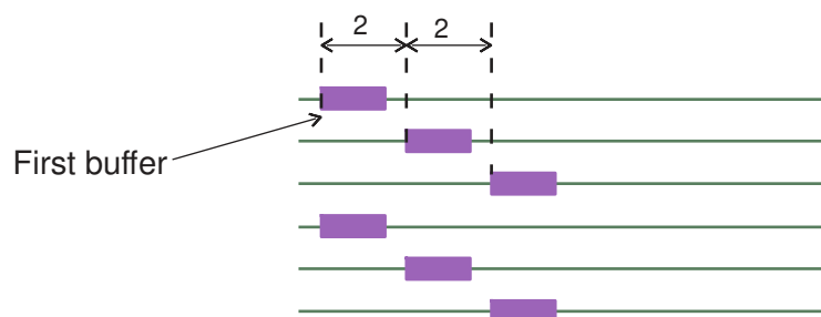
Figure 219 Buffer Patterns for a Horizontal Bus
