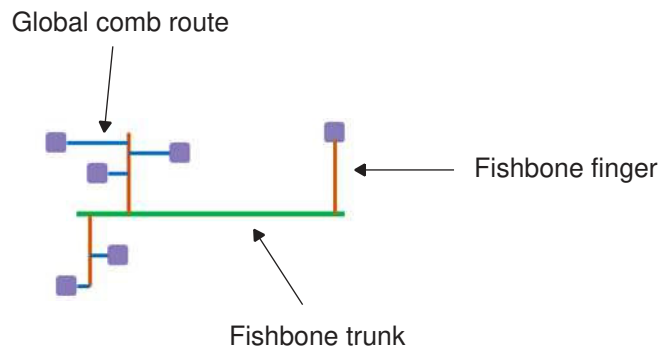
Figure 97 Detail Fishbone Routes and Global Comb Routes
