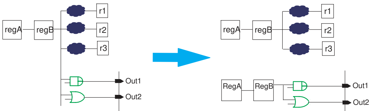
Figure 33 Before and After Register Replication
