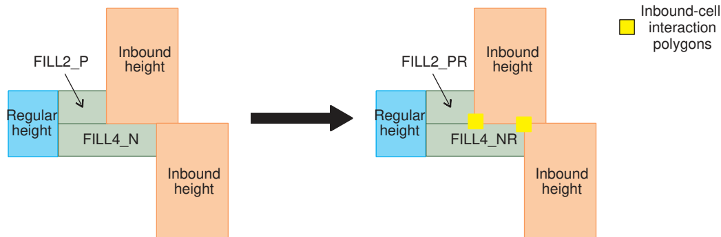
Figure 128 Half-Height Filler Cell Replacement With Half Row Adjacency Rule
