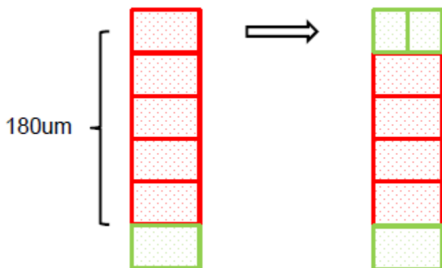
Figure 133 Fixing a Maximum Vertical Edge Length Violation
