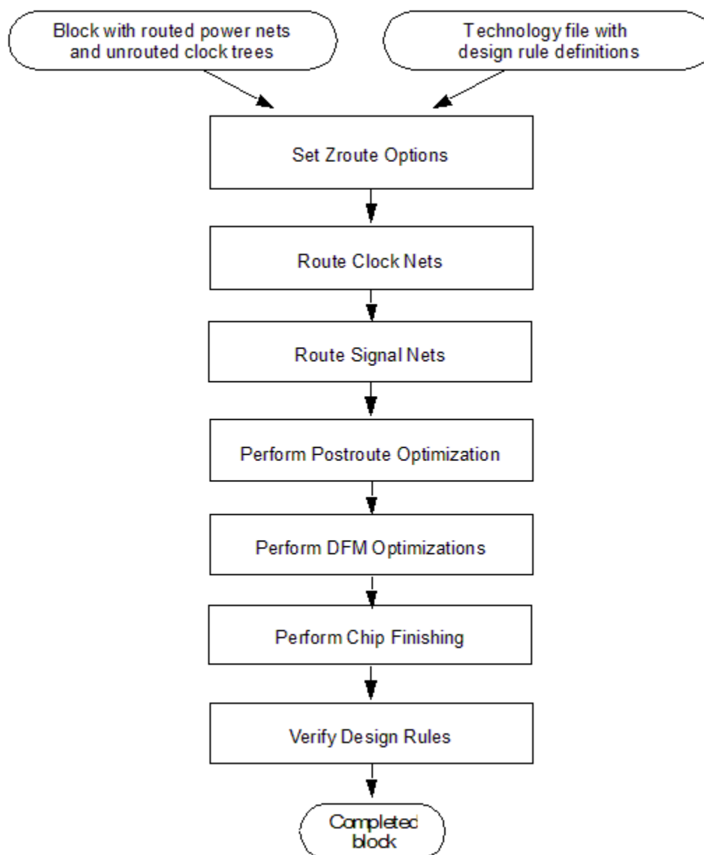
Figure 99 Basic Zroute Flow
