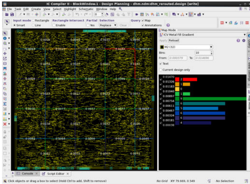
Figure 152 Density Gradient Heat Map
