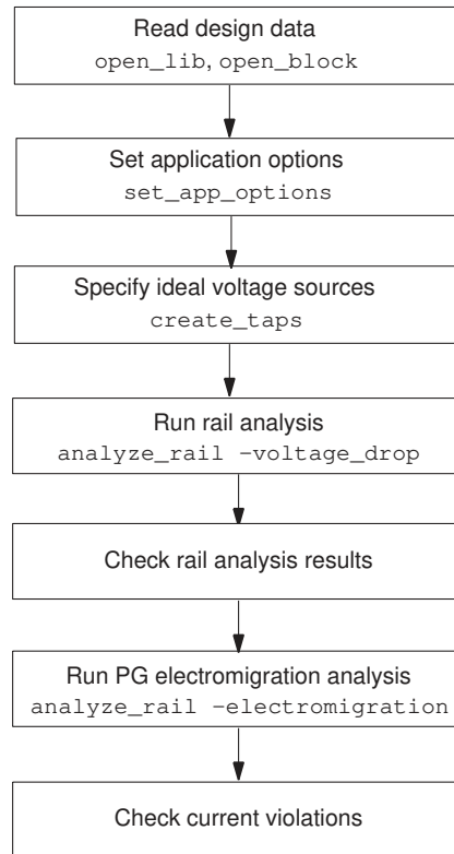
Figure 200 Required Steps for a Basic Rail Analysis Using RedHawk and RedHawk-SC Fusion
