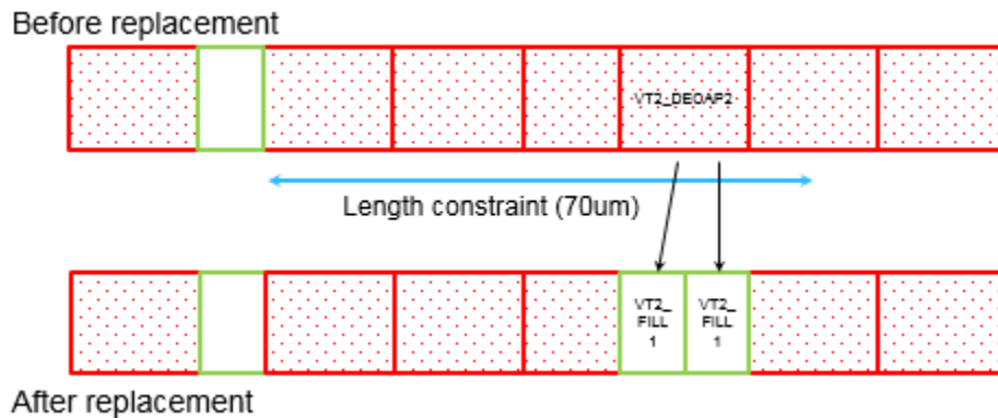
Figure 130 Fixing a Maximum Vertical Edge Length Violation
