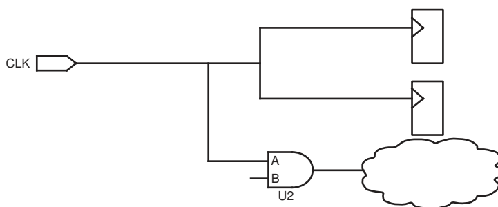
Figure 74 User-Defined Ignore Pin
