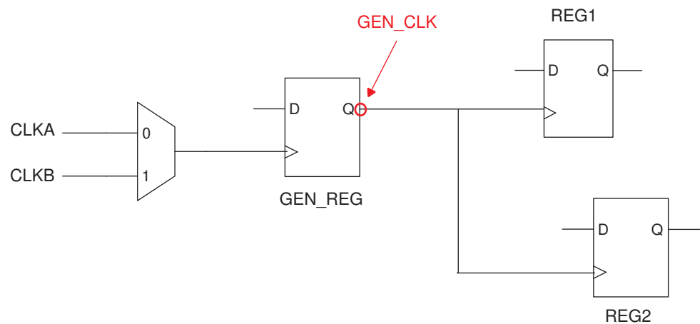
Figure 78 Generated Clock With Invalid Master Clock Source
