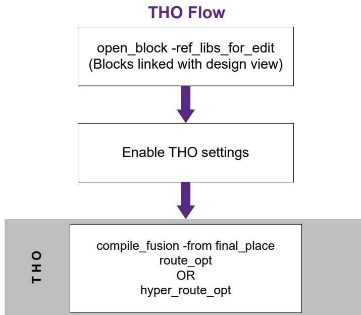
Figure 197 Transparent Hierarchy Optimization Flow
