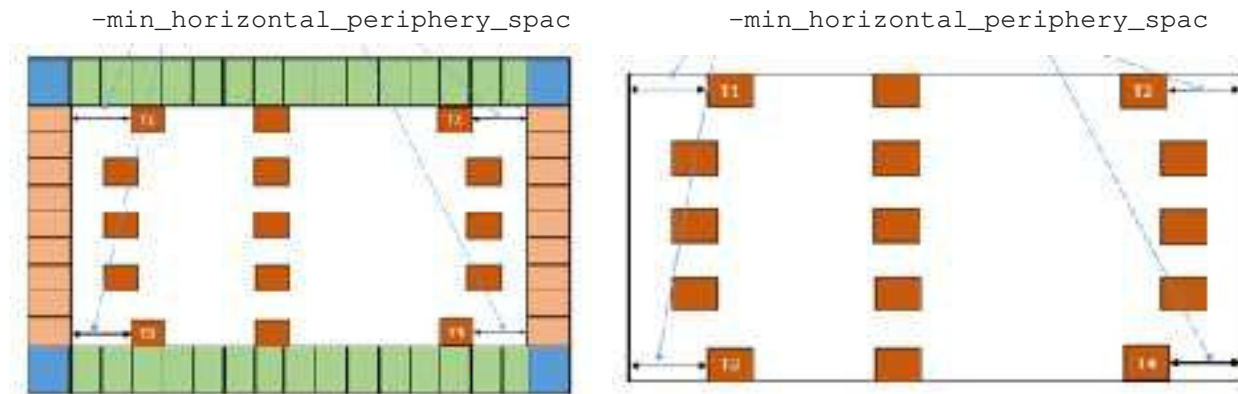
Figure 122 Tap Cell Boundary Row Spacing
