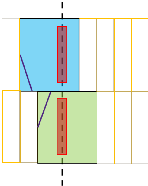
Figure 23 Equivalent Cells With Different Pin Locations
