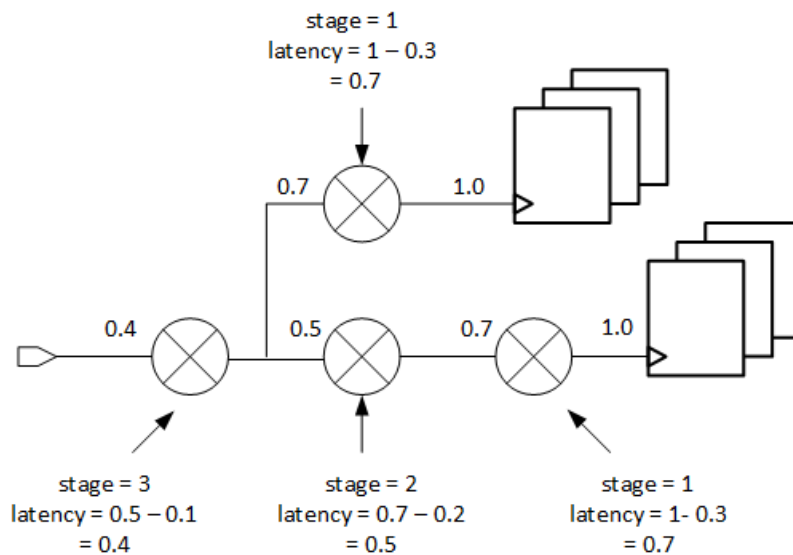
Figure 56 Clock-Gating Stages and Latency Calculations
