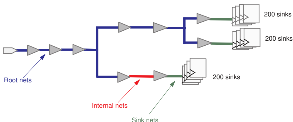
Figure 108 Using a Fanout Limit for Selecting Root Nets
