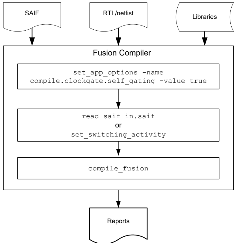
Figure 68 General Self-Gating Flow
