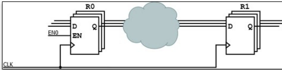
Figure 62 Before Clock Gating
