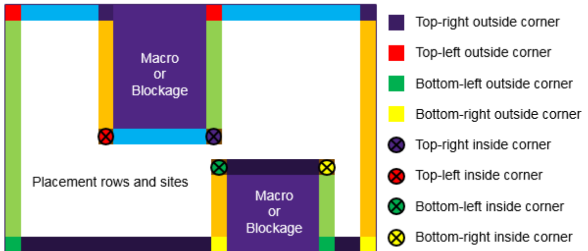
Figure 123 Boundary Cell Locations
