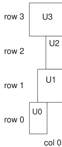
Figure 179 Right-Aligned Relative Placement Group With One Cell That is Left Aligned
