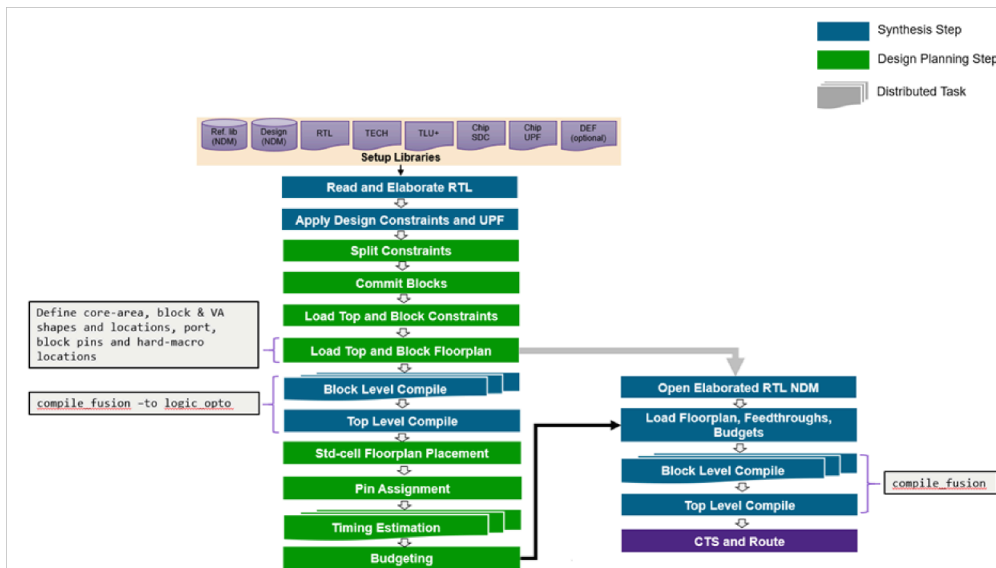
Figure 188 Hierarchical Synthesis Flow When Floorplans are Available
