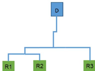
Figure 157 Receivers With Matched Wire Length From Driver D
