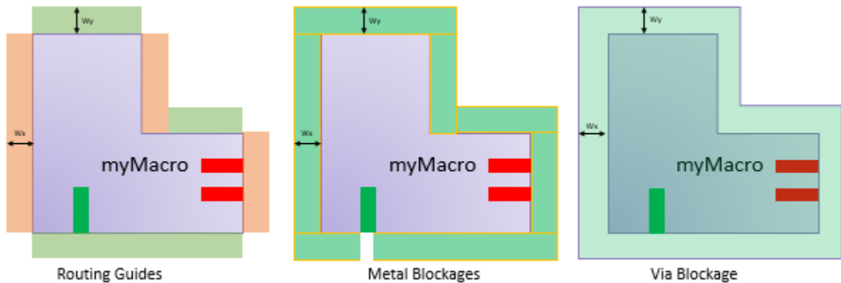
Figure 100 Pin Access Routing Guides and Blockages
