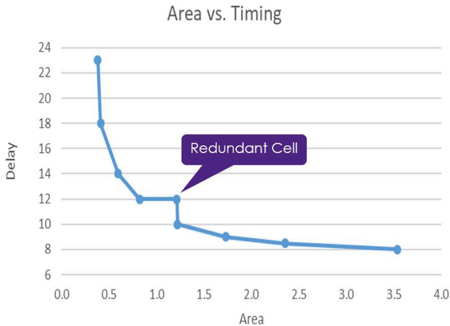
Figure 10 Redundant Cell in Library Cell Family
