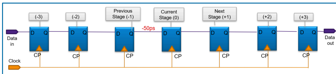
Figure 82 Previous, Current, and Next Path Stages
