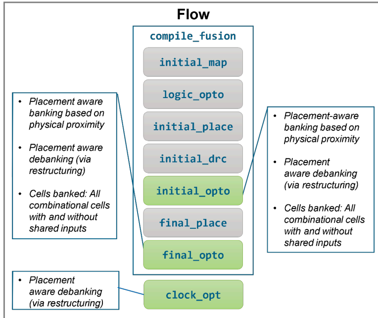
Figure 37 Combinational Multibit Library Cell Flow
