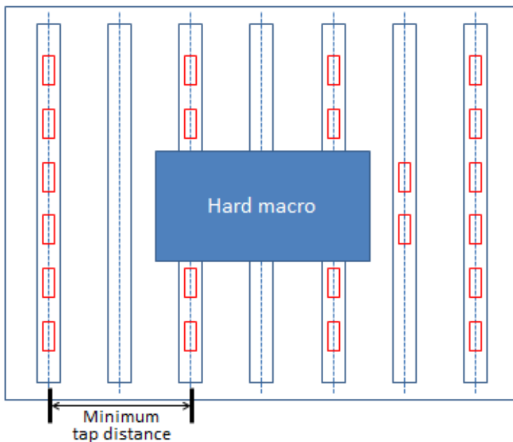
Figure 121 Default Tap Cell Placement
