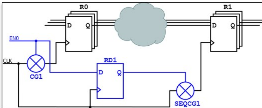
Figure 63 After Clock Gating
