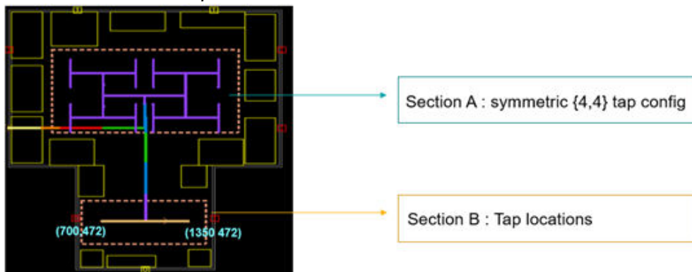
Figure 87 MSCTS Multiple H-Tree
