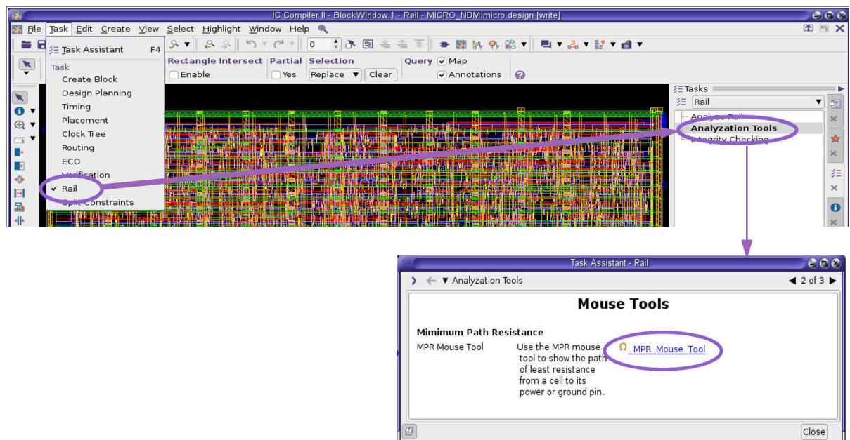
Figure 208 Invoking the MPR Mouse Tool
