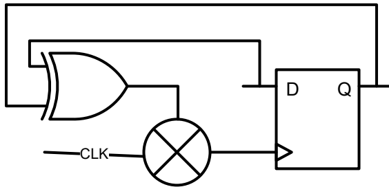
Figure 66 Example of a Self-Gating Cell
