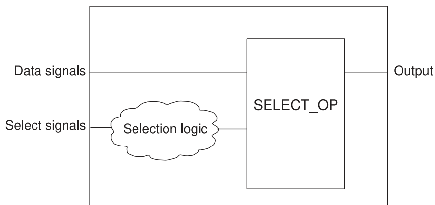
Figure 32 Verilog Output—SELECT_OP and Selection Logic
