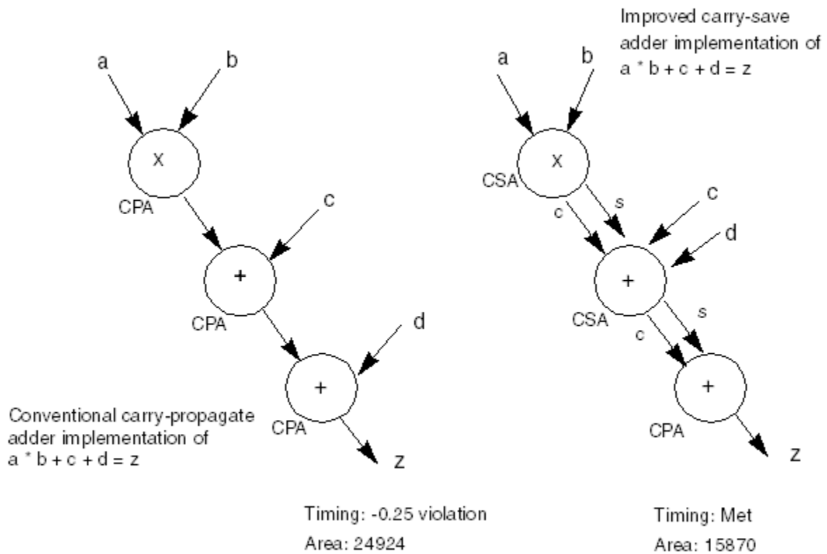
Figure 30 Conventional Carry-Propagate Adder Versus Carry-Save Adder
