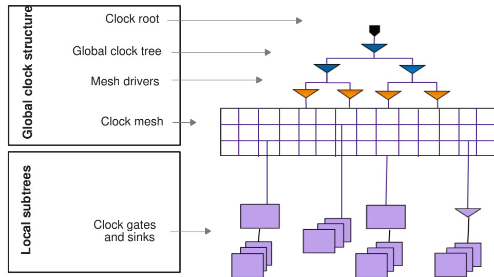
Figure 84 Structural Multisource Clock Tree
