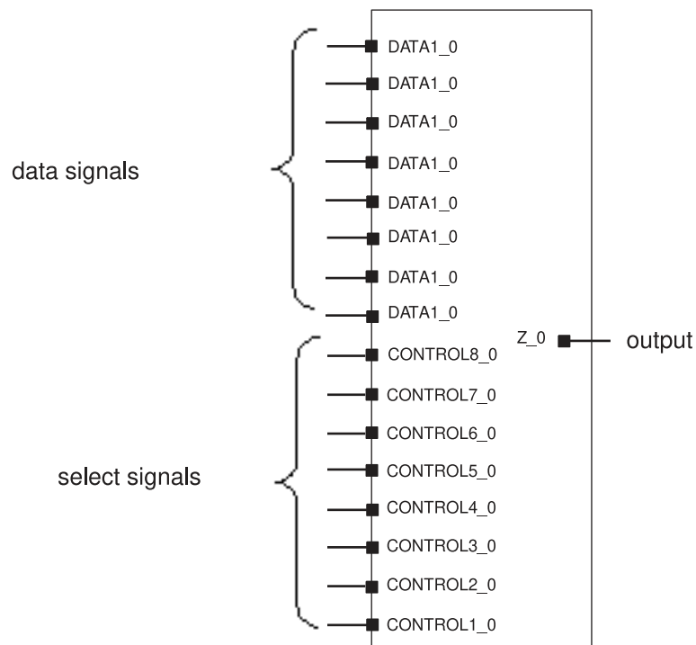
Figure 31 SELECT_OP Implementation for an 8-bit Data Signal
