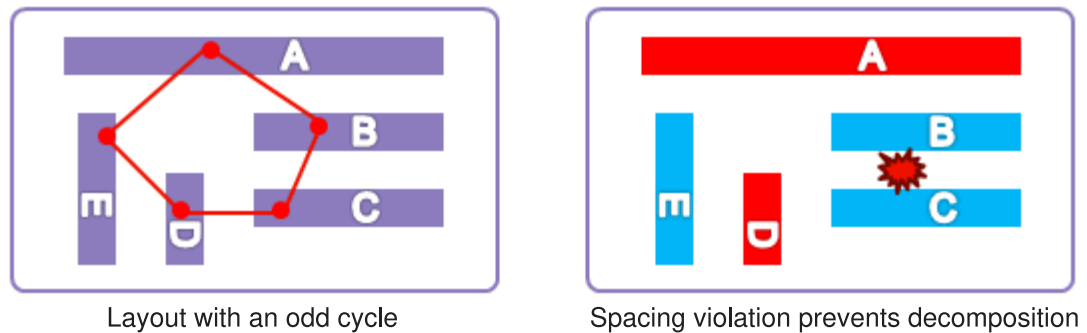
Figure 5 Odd-Cycle Violation
