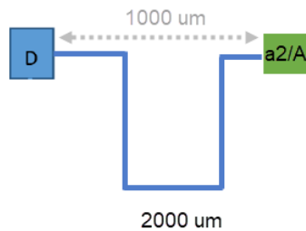
Figure 156 Minimum Wire Length Constraint for the a2/A Pin
