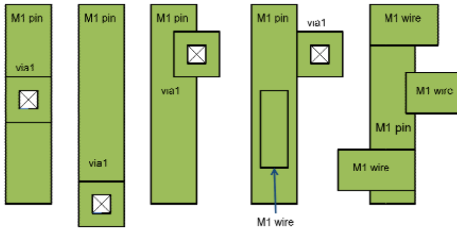
Figure 113 Unrestricted Pin Connections
