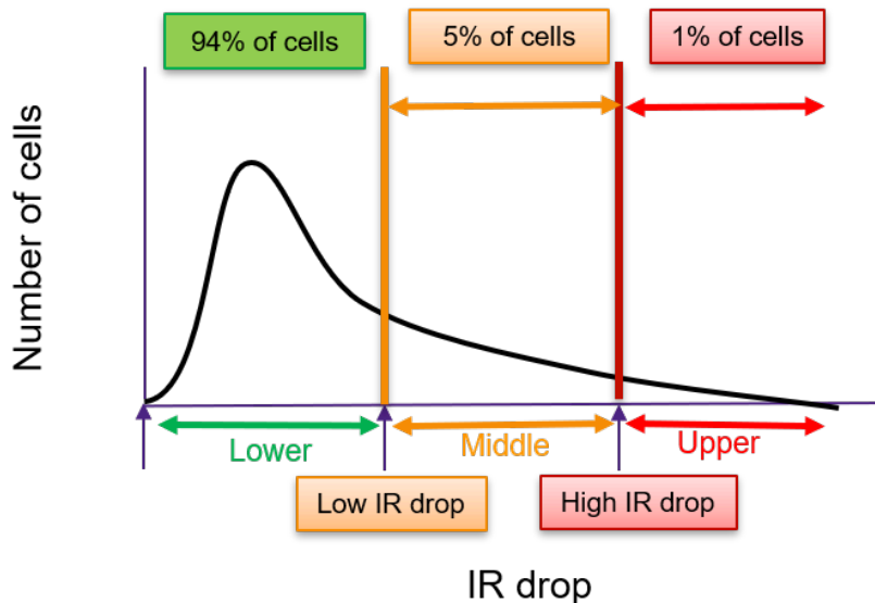
Figure 22 Default Cell Categories for IR-Drop-Aware Placement
