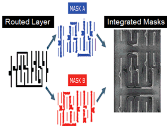
Figure 4 Double-Patterning Example
