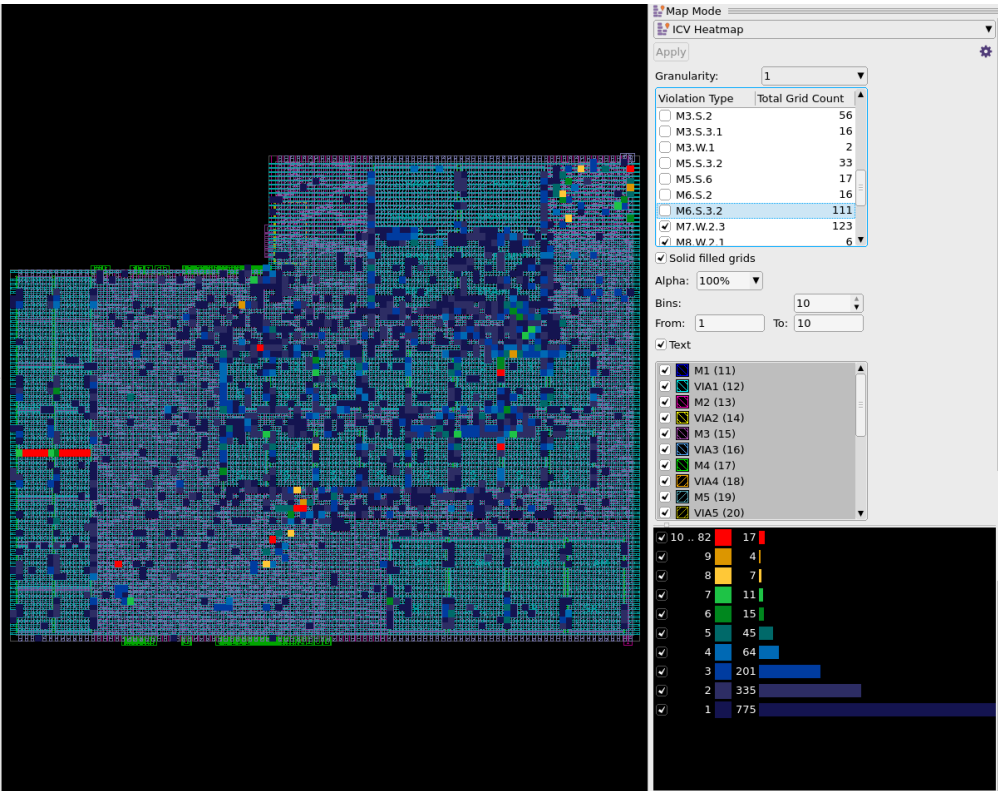
Figure 137 Violation Type in ICV Heat Map
