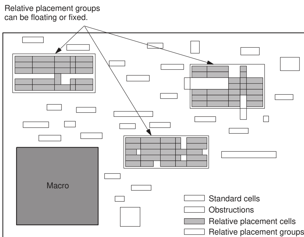
Figure 166 Relative Placement in a Floorplan
