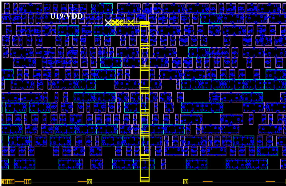
Figure 207 Traced Segment is Highlighted in the Design Layout
