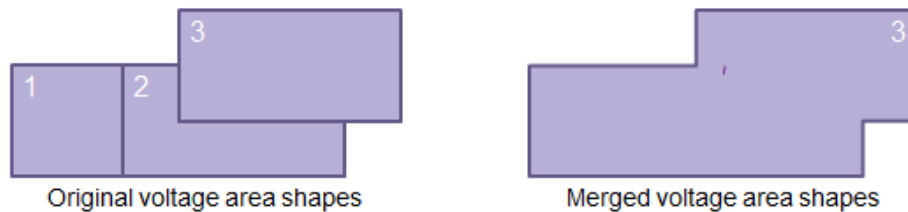
Figure 14 Merging Voltage Area Shapes
