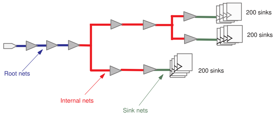
Figure 107 Root, Internal, and Sink Clock Net Types
