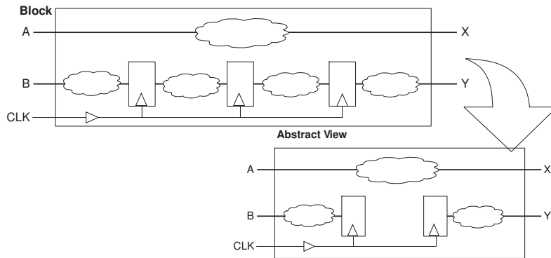
Figure 191 A Block and Its Abstract View
