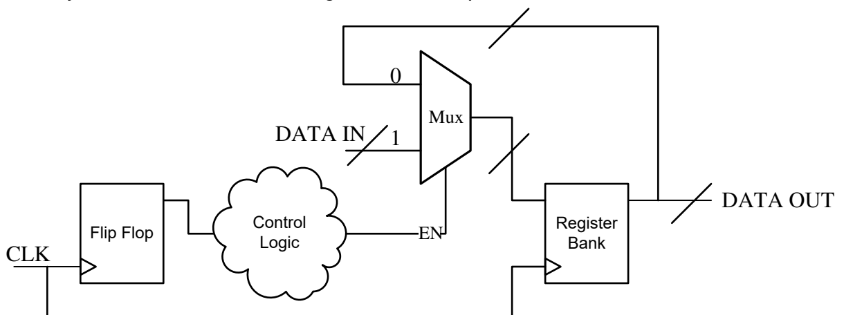
Figure 45 Synchronous Load-Enable Register With Multiplexer
