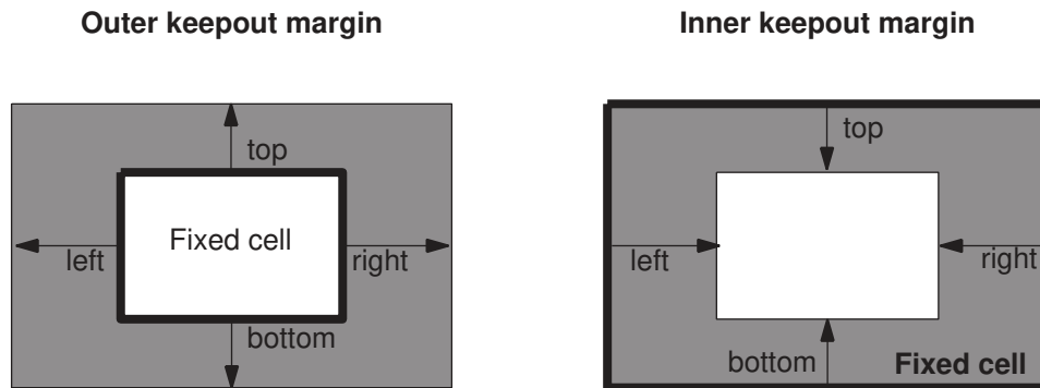
Figure 21 Placement Keepout Margins
