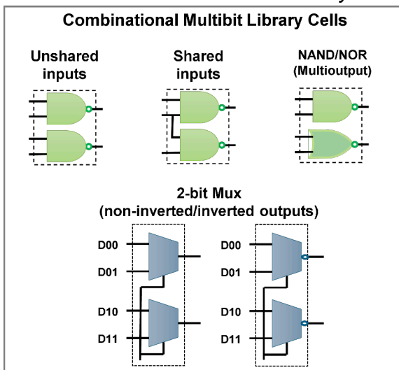
Figure 36 Combinational Multibit Library Cells
