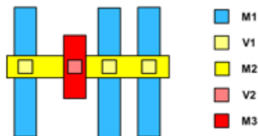
Figure 111 Multi-Level Pattern-Based Must-Join Pin Connection
