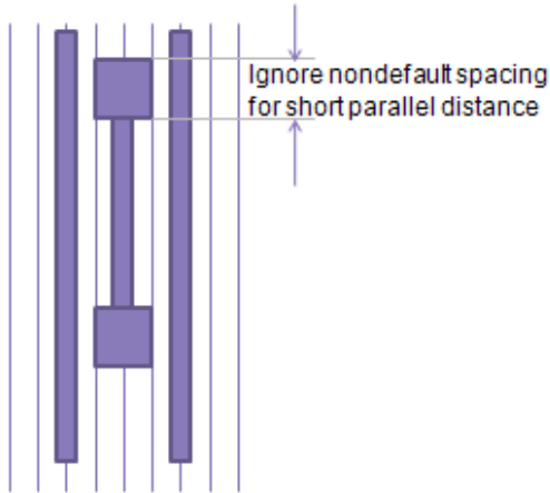
Figure 106 Ignoring Nondefault Spacing Rule Violations
