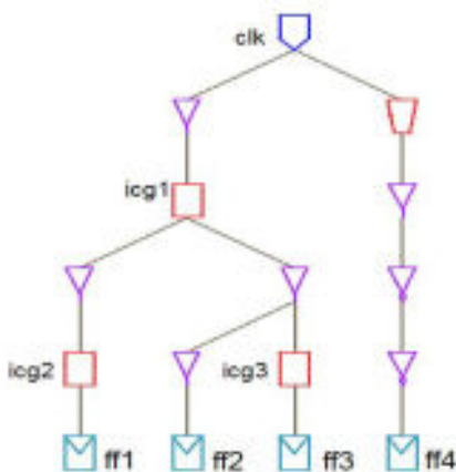
Figure 98 Segments and Subtrees of a Clock Tree
