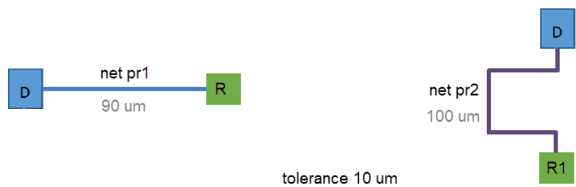
Figure 159 Net-Based Wire Length Matching
