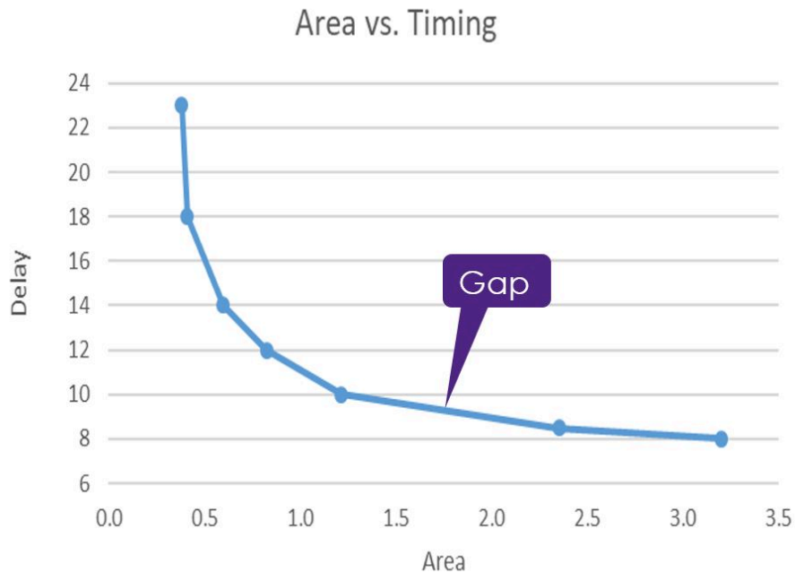
Figure 13 Gap in Library Cell Family
