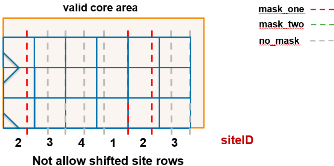
Figure 227 Calculation for Variant siteId
