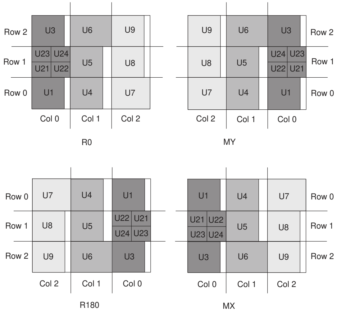
Figure 182 Orientation of Relative Placement Groups
