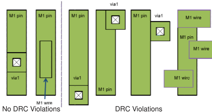
Figure 115 Restricted Via-to-Pin and Wire-to-Pin Connections
