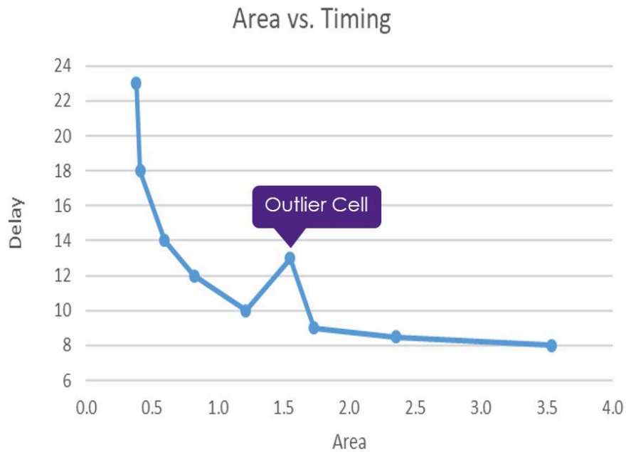
Figure 11 Outlier Cell in Library Cell Family
