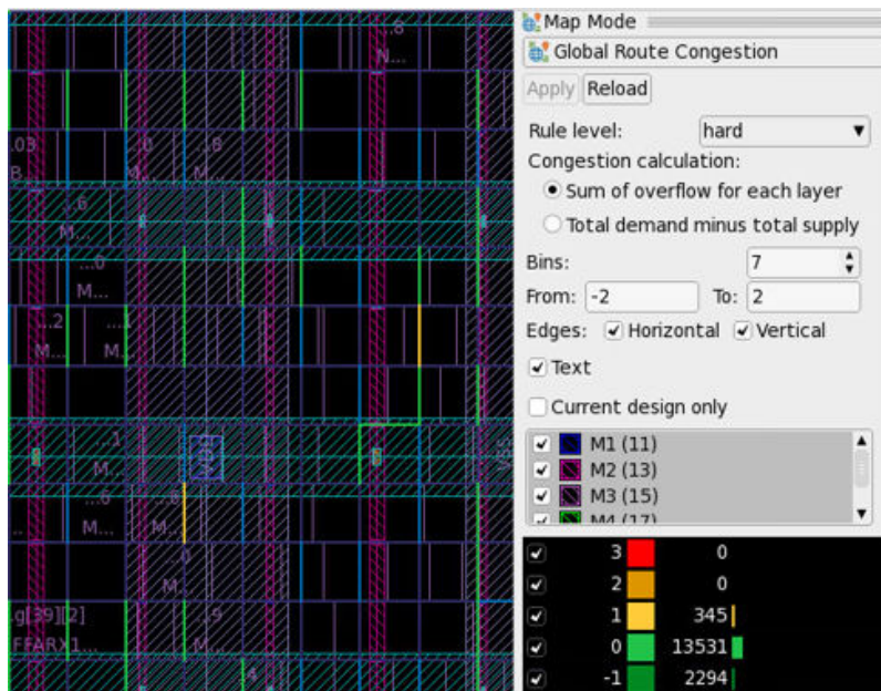
Figure 118 Global Route Congestion Map
