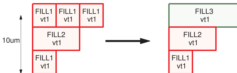
Figure 131 Fixing Maximum Stacking Violation by Replacement
