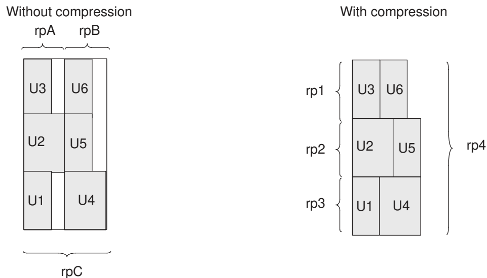
Figure 171 Bottom-Left Alignment Construction and Compression
