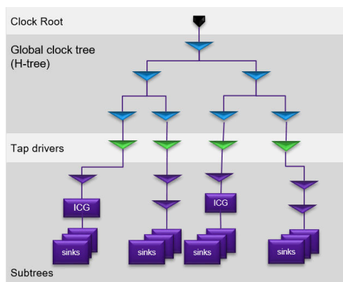
Figure 85 Regular Multisource Clock Tree With an H-Tree-Only Global Clock Structure
