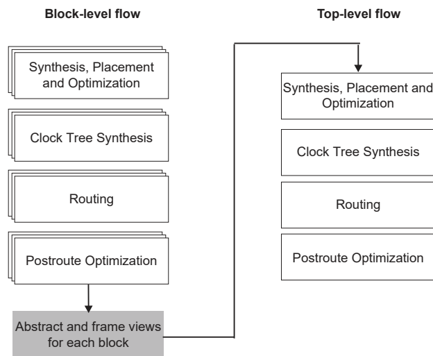
Figure 195 Top-Level Implemented After Blocks are Completed
