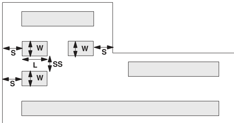
Figure 103 Metal Shape Perimeter Constraint Objects With Additional Short Shapes
