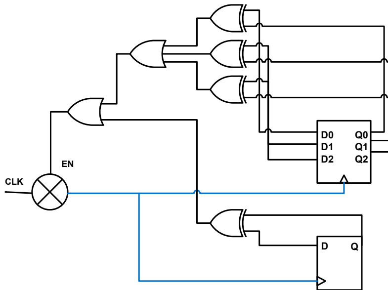
Figure 67 Self-Gating Tree
