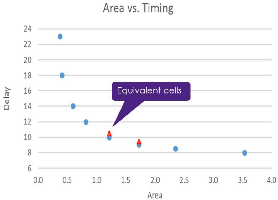
Figure 12 Equivalent Cells in Library Cell Family
