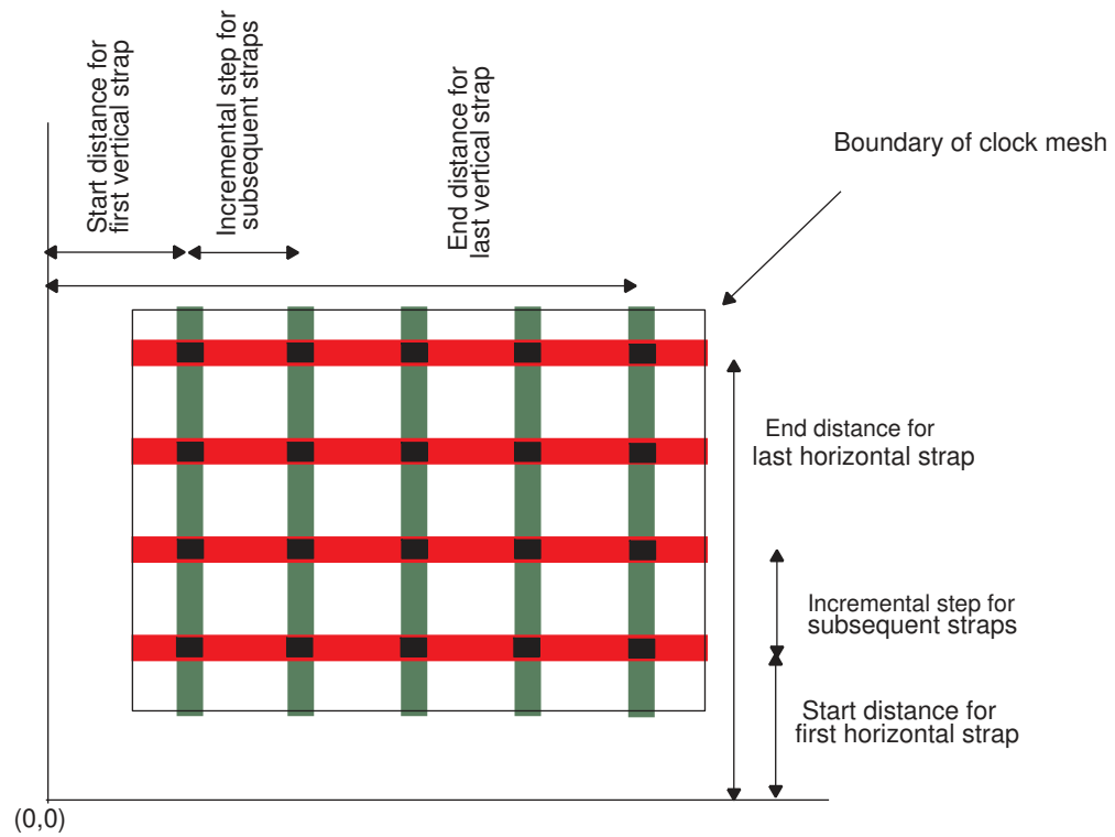
Figure 89 Clock Mesh Structure
