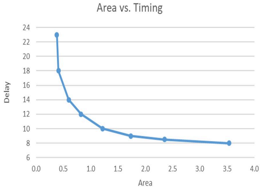
Figure 9 Monotonic Distribution in Library Cell Family
