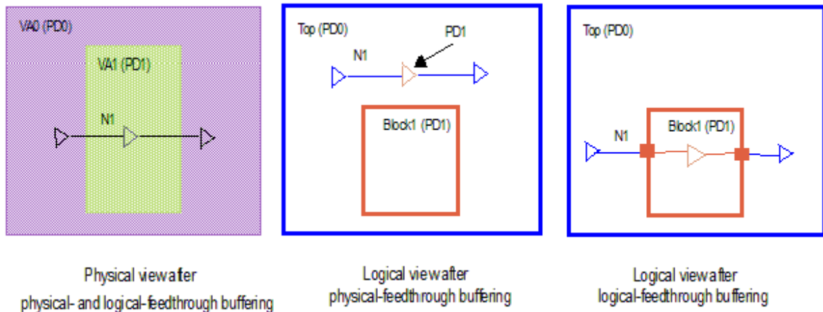
Figure 20 Difference in the Logical View After Physical- and Logical-Feedthrough Buffering
